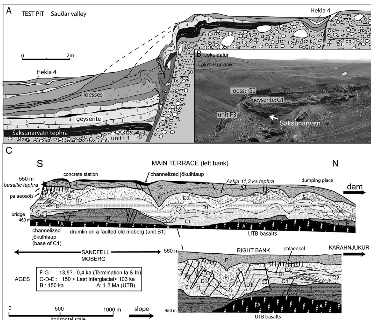
Fig. 5. Deformation structures.
